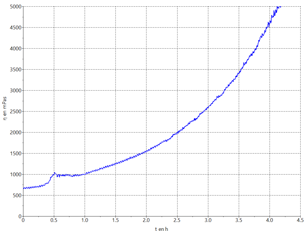
HTG-240 mixed viscosity evolution at 23 °C
